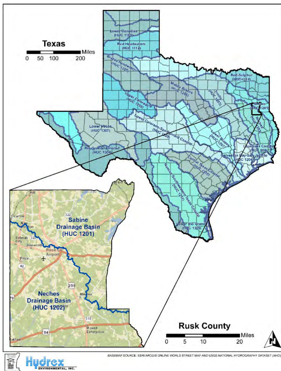
Figure 15. Major drainage basins within Texas and Rusk County.
